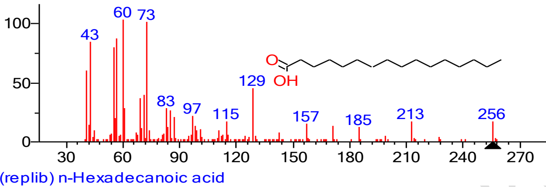
Figure 8. Spectra of n-Hexadecanoic acid
